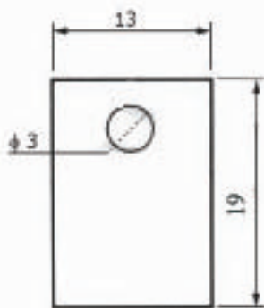
TO-220
