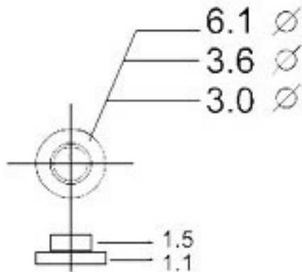
TO-220
