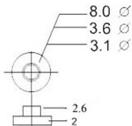
TO-218
