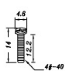
(STF-4*12.5)*2
